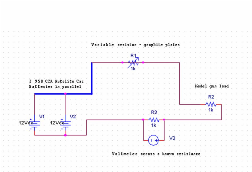
Figure 17. The subtle change here is the removal of the 1kA equivalent fuse. This allowed us to progressively increase the current to a maximum value of 3400A.
